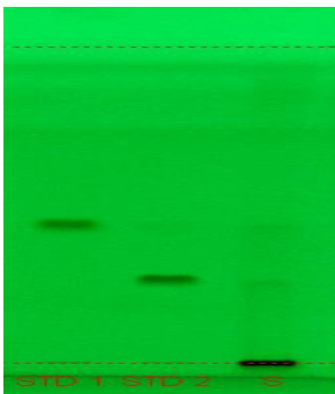
Figure 2: HPTLC chromatograms of Strychnos Nux-vomica at 254nm.
