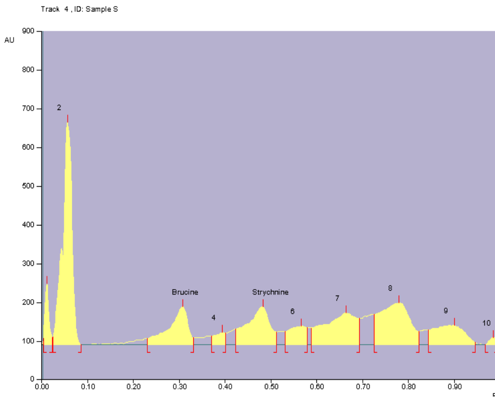
Figure 1: HPTLC chromatograms shows the compounds of Strychnos Nux-vomica .
