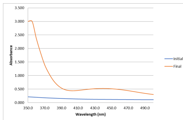
Figure 2: UV –Vis Spectroscopy of Ginger oil mediated silver nanoparticles
