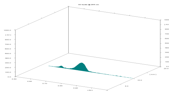
Figure 3: Densitogram of standard solution of Amlodipine Besylate and Olmesartan Medoxomil
