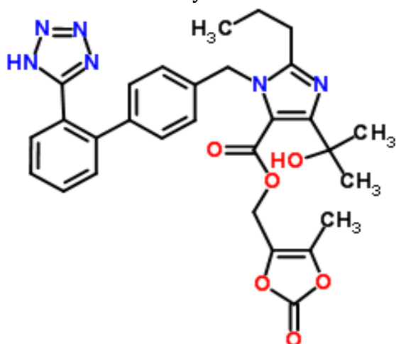
Figure 2: Chemical structures of Olmesartan medoxomil
