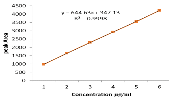
Figure 5: Linearity plot of Amlodipine besylate
