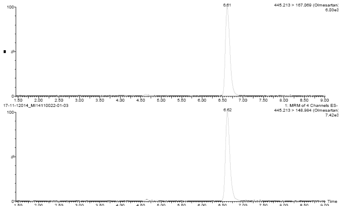
Figure 10: MRM ion-chromatograms of Olmesartan
