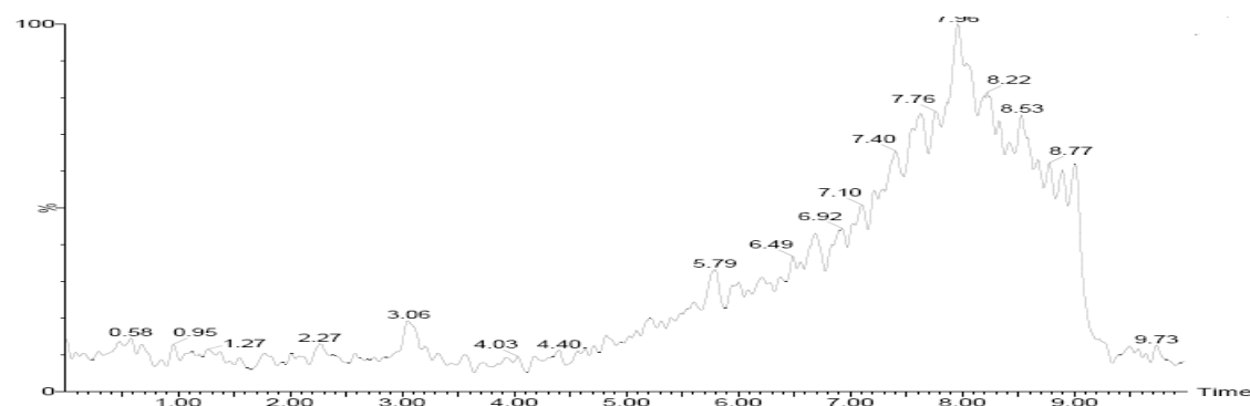
Figure 9: MRM ion-chromatograms of Double blank plasma (without IS) negative ion mode
