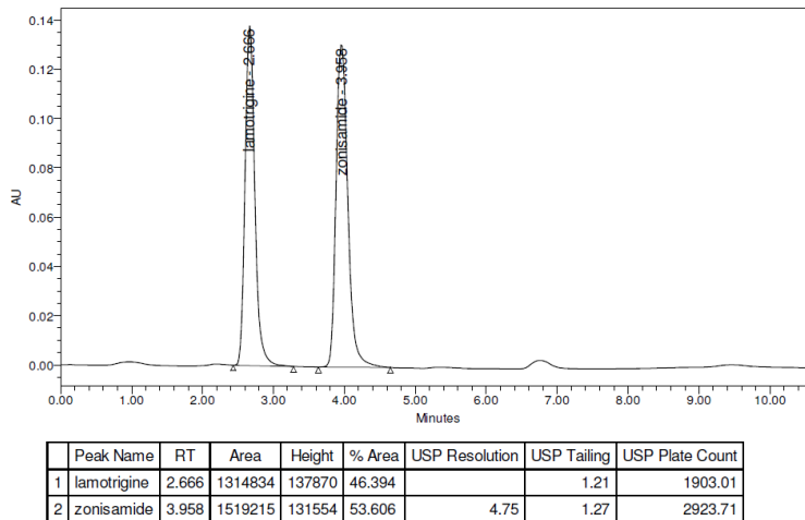
Figure 6: Standard Chromatogram of Lamotrigine and Zonisamide
