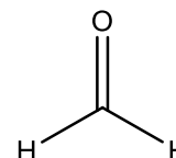
Figure 1: Structure of Formaldehyde
