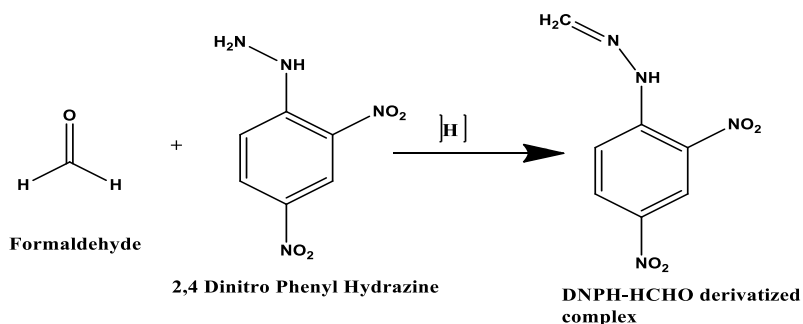
Figure 2: Derivatization of DNP-HCHO complex reaction scheme
